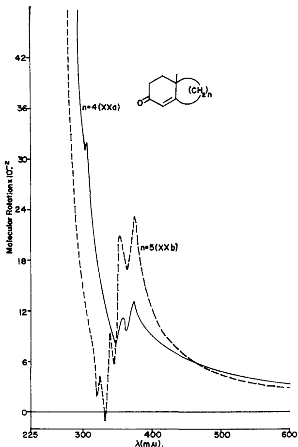
Fig. 2.—Optical rotatory dispersion curves (dioxane solution) of \Delta^{1(9)} -10-methyl-2-octalone (XXa) and \Delta^2 -1 \beta -methylbicyclo[5.4.0]-9-undecenone (XXb).
